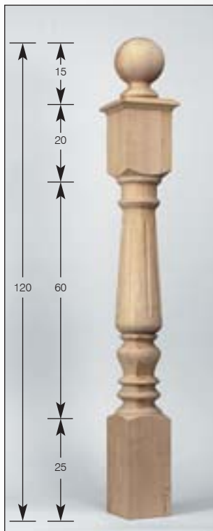
Extra heavy baluster / Antrittsposten / Balustre / Aanvangs baluster Art.Nr. 50.0150.012.00 ∅ 12 cm
