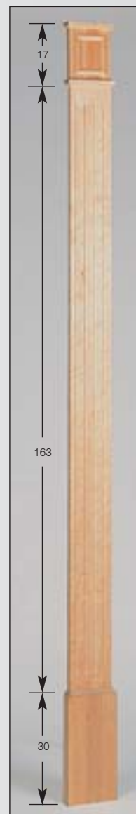
Art.Nr. 50.2460.210.00 H 210 cm Top B 14, T 3,5 cm Base B 14, T 3,5 cm
