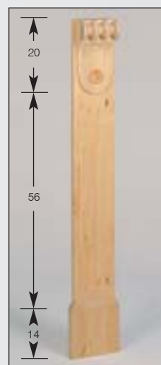
Art.Nr. 50.2310.090.00 H 90 cm Top B 12, T 7 cm Base B 14, T 2,5 cm
