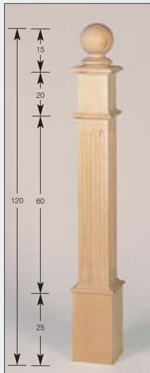
Extra heavy baluster / Antrittsposten / Balustre / Aanvangs baluster Art.Nr. 50.0350.015.00 ∅ 15 cm
