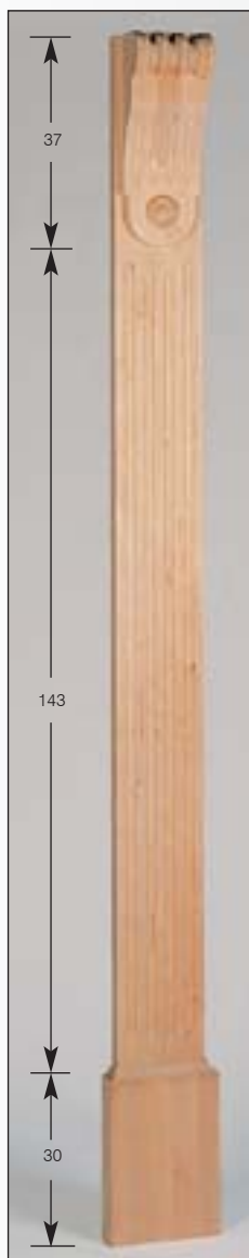
Art.Nr. 50.2370.210.00 H 210 cm Top B 16, T 13,5 cm Base B 20, T 5 cm
