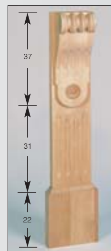
Art.Nr. 50.2320.090.00 H 90 cm Top B 16, T 14 cm Base B 20, T 5 cm
