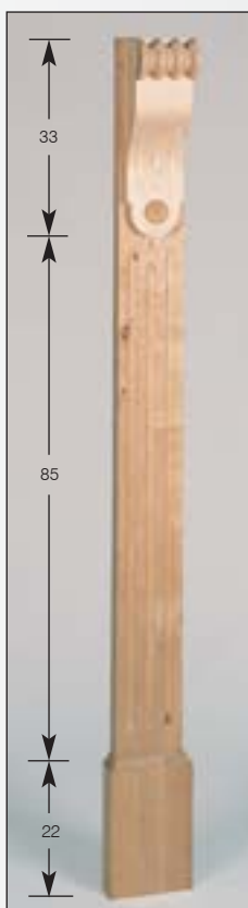
Art.Nr. 50.2340.140.00 H 140 cm Top B 11,5, T 13 cm Base B 14, T 5 cm
